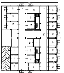
505 5th Floor Plan (1/10/2018)
