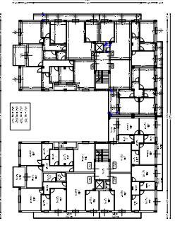
505 5th Floor Plan (1/10/2018)
